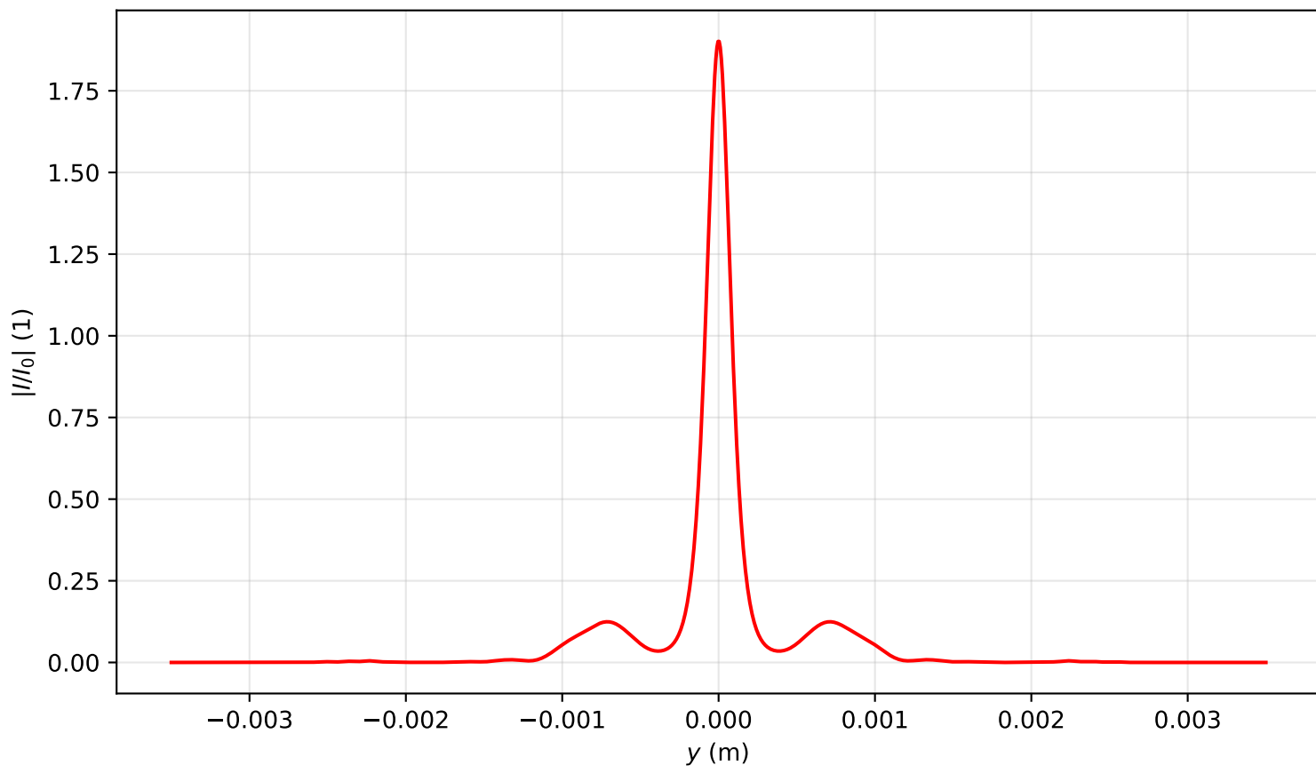
Intensity profile I(x=0, y, z=1.672)/I_0 , P_{in}=8.0P_{cr} , artificial time
